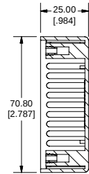
SECTION B-B
