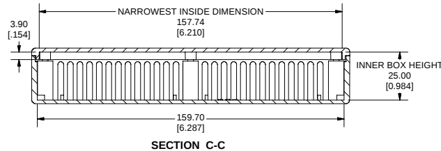
SECTION C-C
